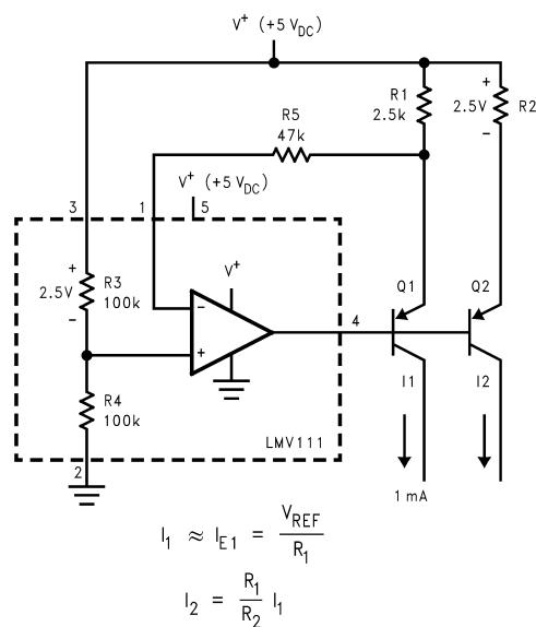
FIGURE 3. Fixed Current Source
