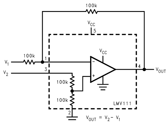
FIGURE 4. Difference Amplifier
